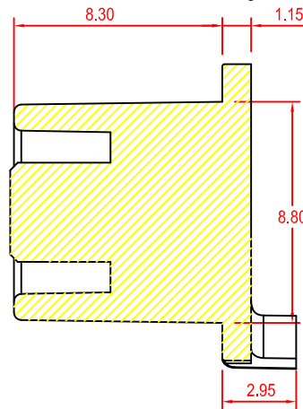
Section 1-1
